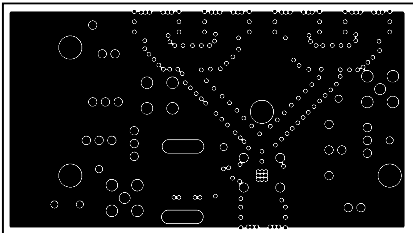
Figure 6. MAX3941 EV Kit PC Board Layout—Power Plane
